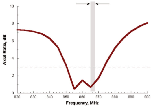
Axial Ratio
