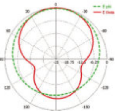
phi = 90
