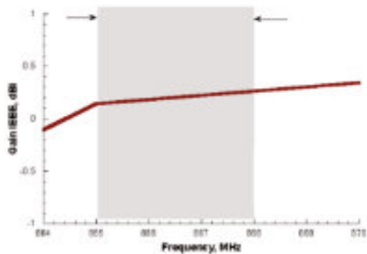
Antenna Gain
