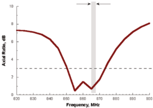
Axial Ratio
