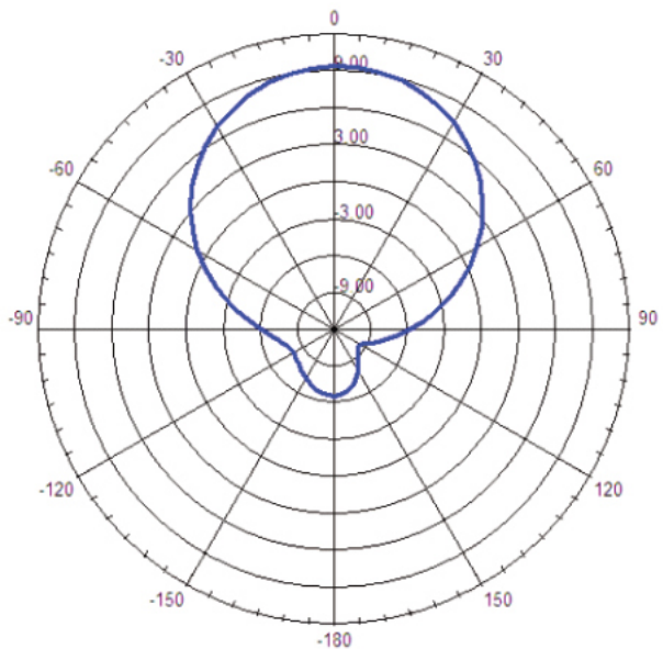
Total Gain - Azimuth
